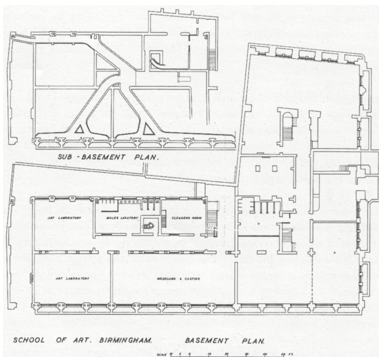
Figure 8. Plan of the extension basement, indicating location of duct system, Birmingham School of Art. (Image: courtesy of Urban Design, Birmingham City Council)
