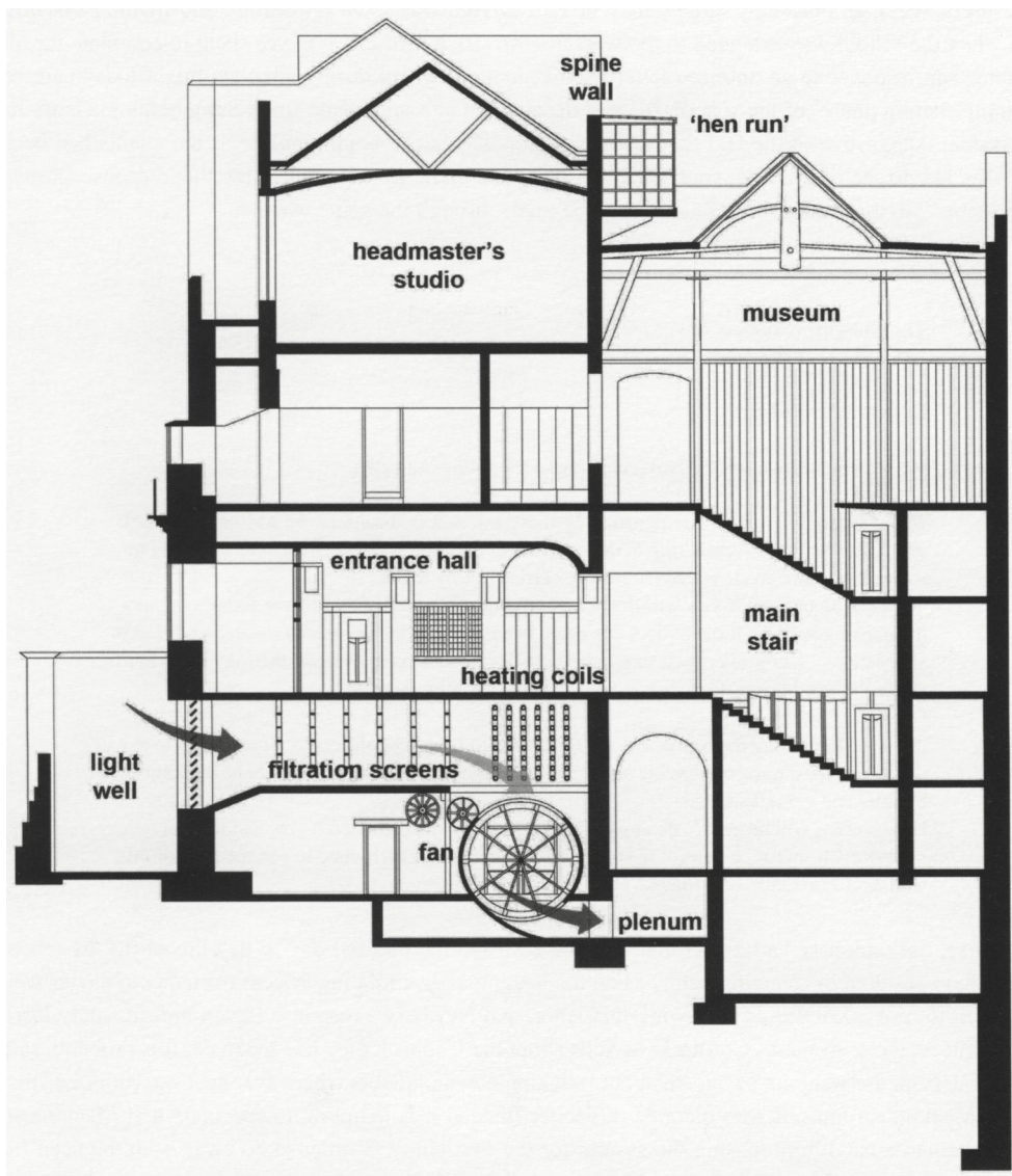
Figure 11. Section detailing fan installation and main plenum, Glasgow School of Art.
