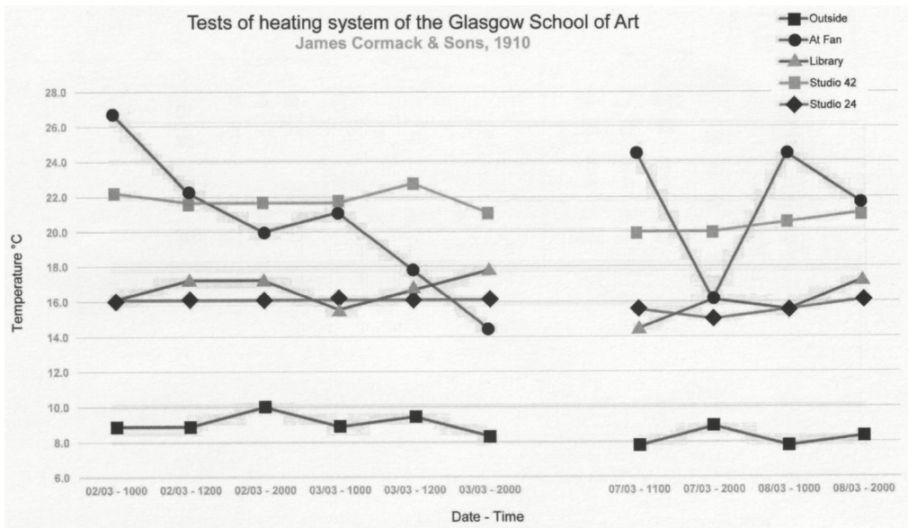
Figure 12. Tests of heating system of the Glasgow School of Art.
